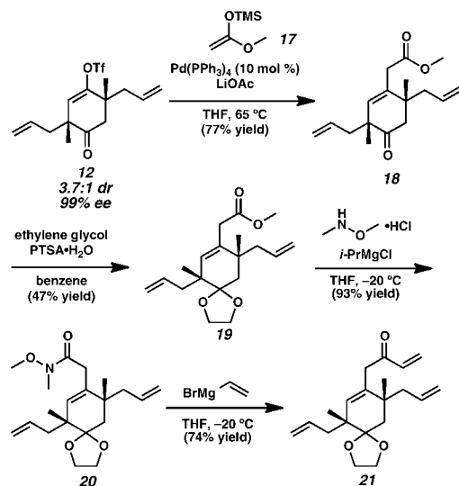
Scheme 3. Synthesis of Enone 21
