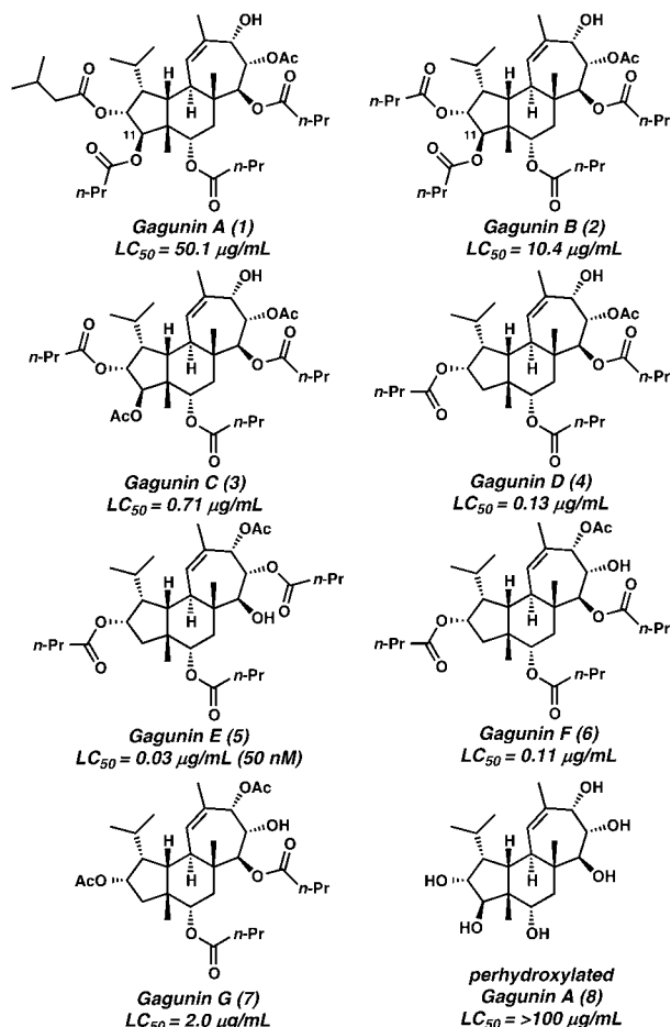
Figure 1. Gagunins A–G (1–7) and perhydroxylated gagunin A (8) and their reported biological activities.
