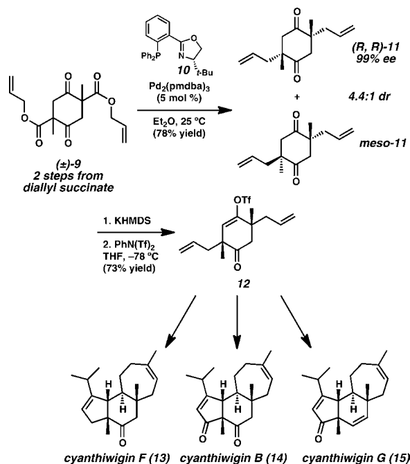
Scheme 1. Enantioselective Tsuji Allylic Alkylation Applied to the Synthesis of Cyanthiwigins F ( 13 ), B ( 14 ), and G ( 15 )
